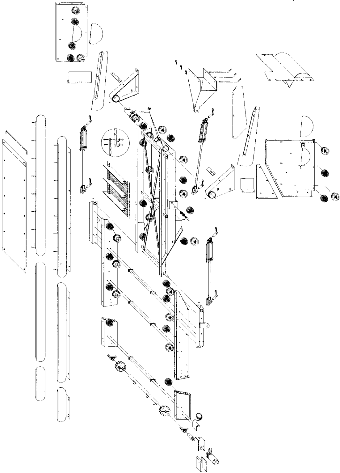
Discharge Conveyor Assembly 194FIG110-1
