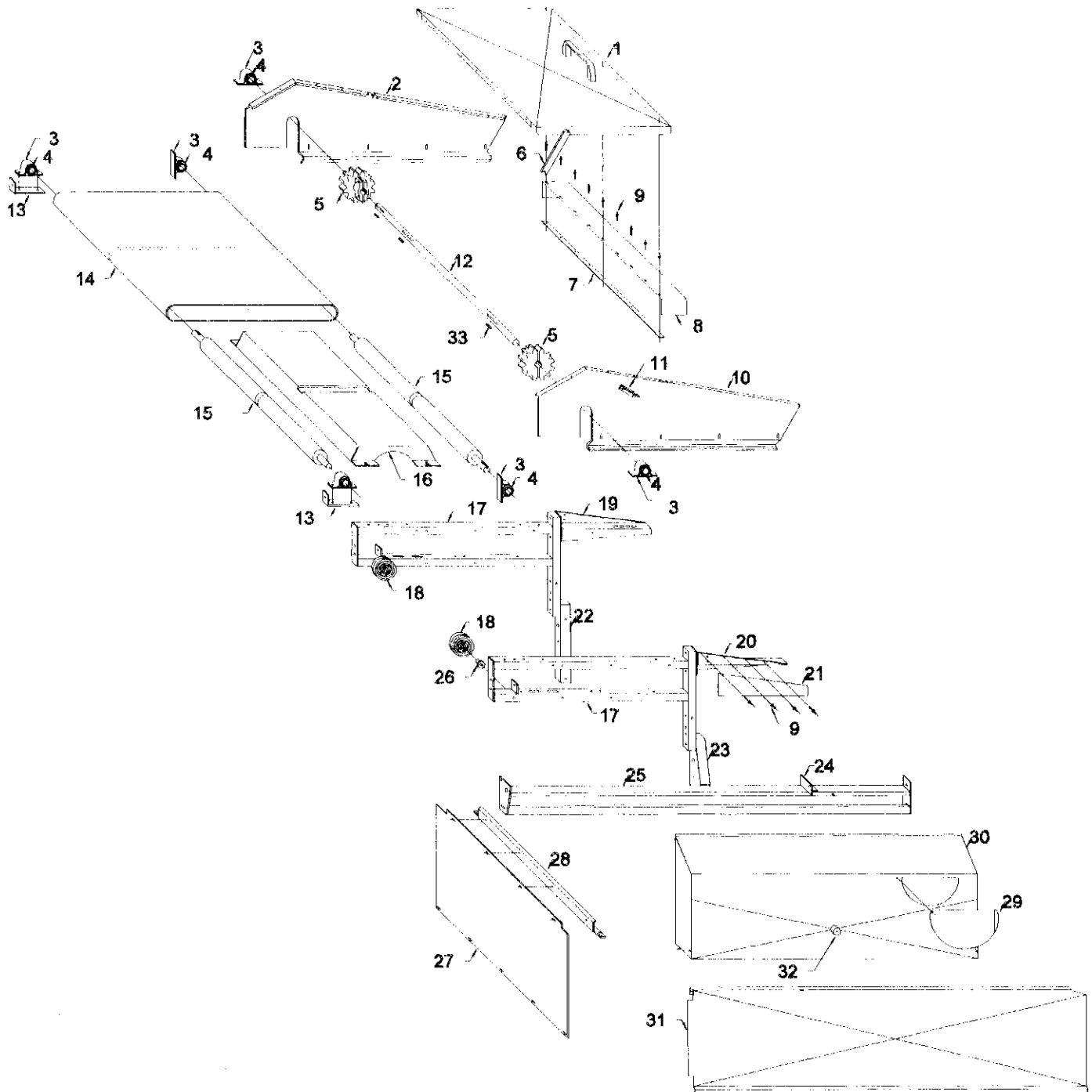
Presort Assembly 194FIG116-1
