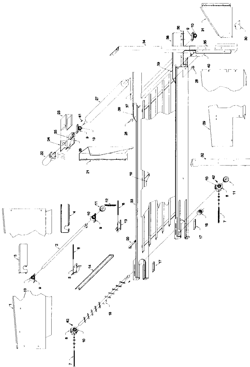
Aftersort Assembly 194FIG17-1
