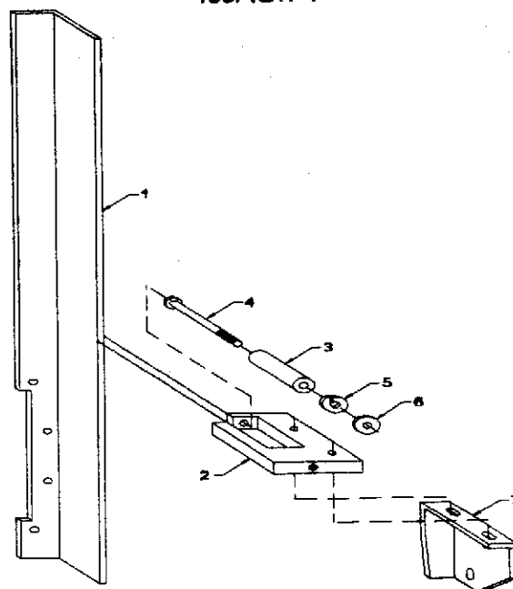
Header Slide Guide Mount Assembly 195FIG1-4
