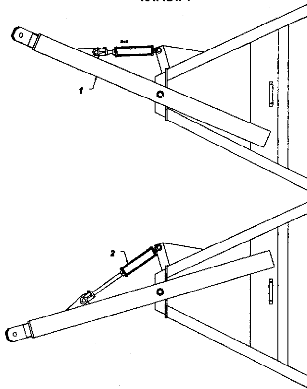
Sliding Hitch Assembly 194FIG4-1
