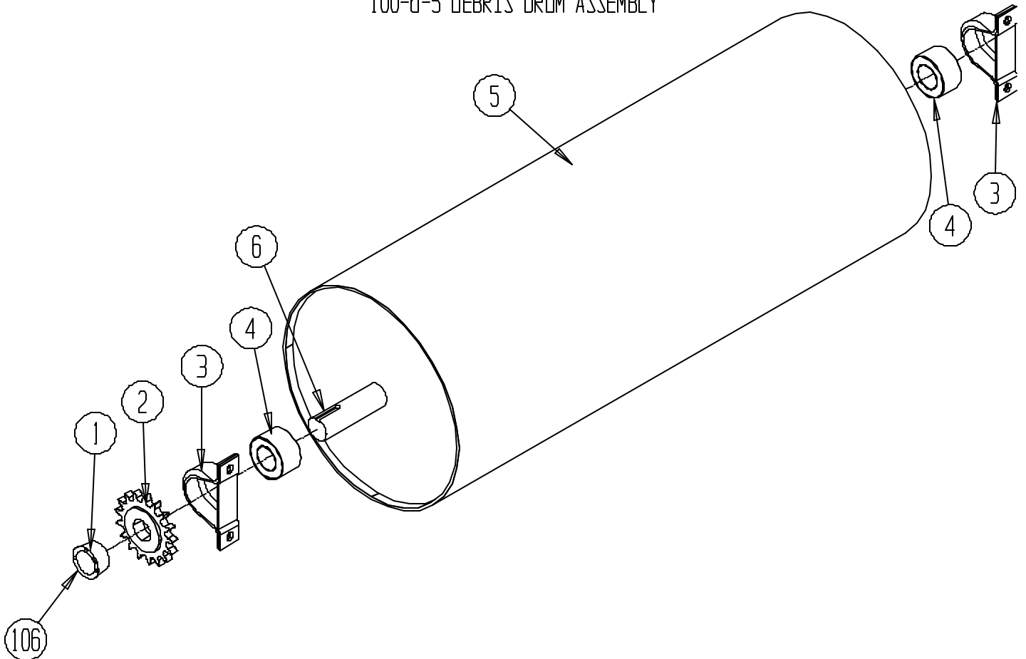
100-6-5 DEBRIS DRUM ASSEMBLY
