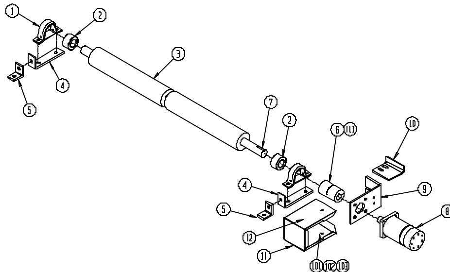
100-8-3 REAR PRESORT ROLLER ASSY.
