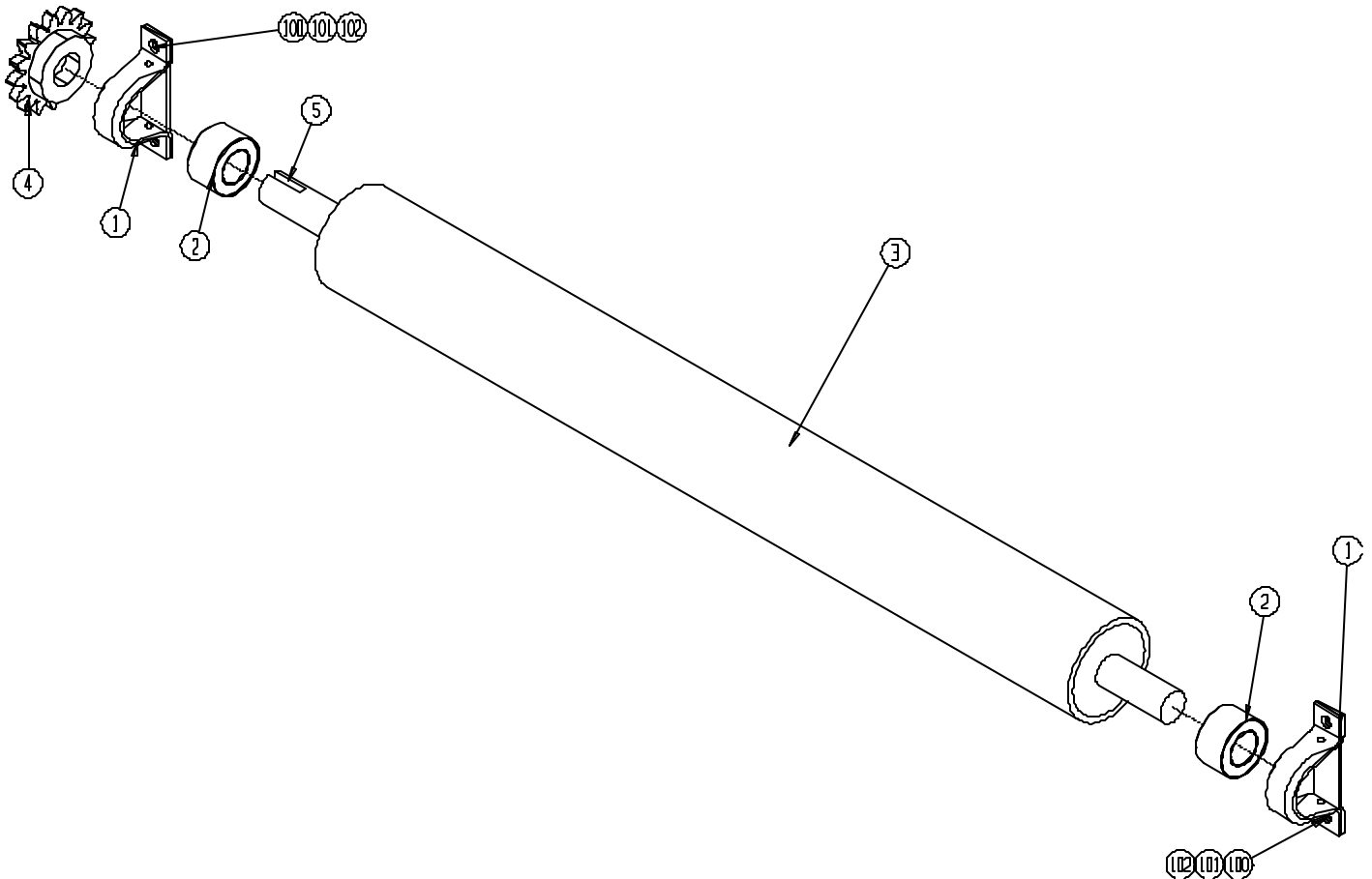
100-2-7 HEADER ROLLER ASSEMBLY
