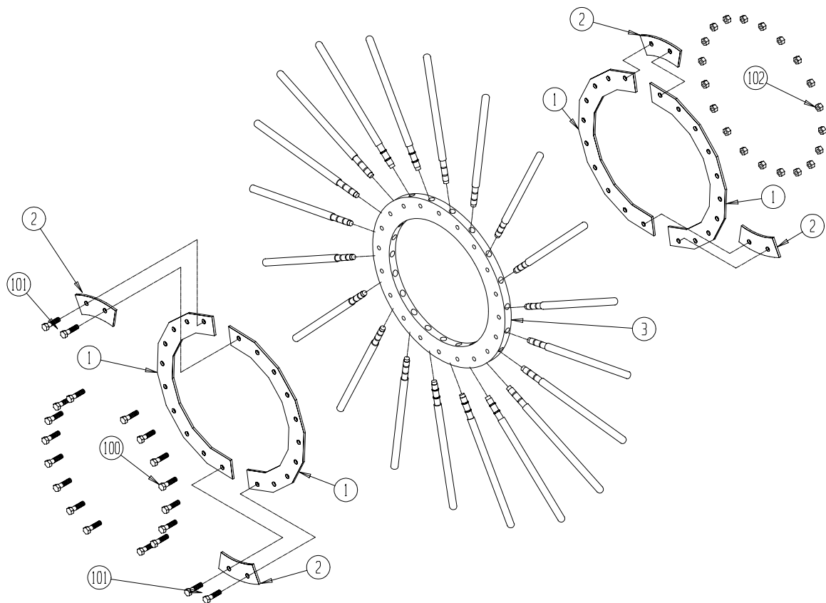
1001-3-10 SHAKER HALF-RING & FINGER ASSEMBLY ( KIT-0091 )
