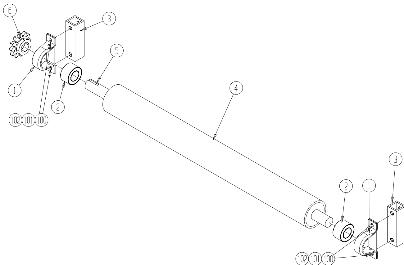
1001-6-3 CROSS CONVEYOR RETURN ROLLER ASSEMBLY
