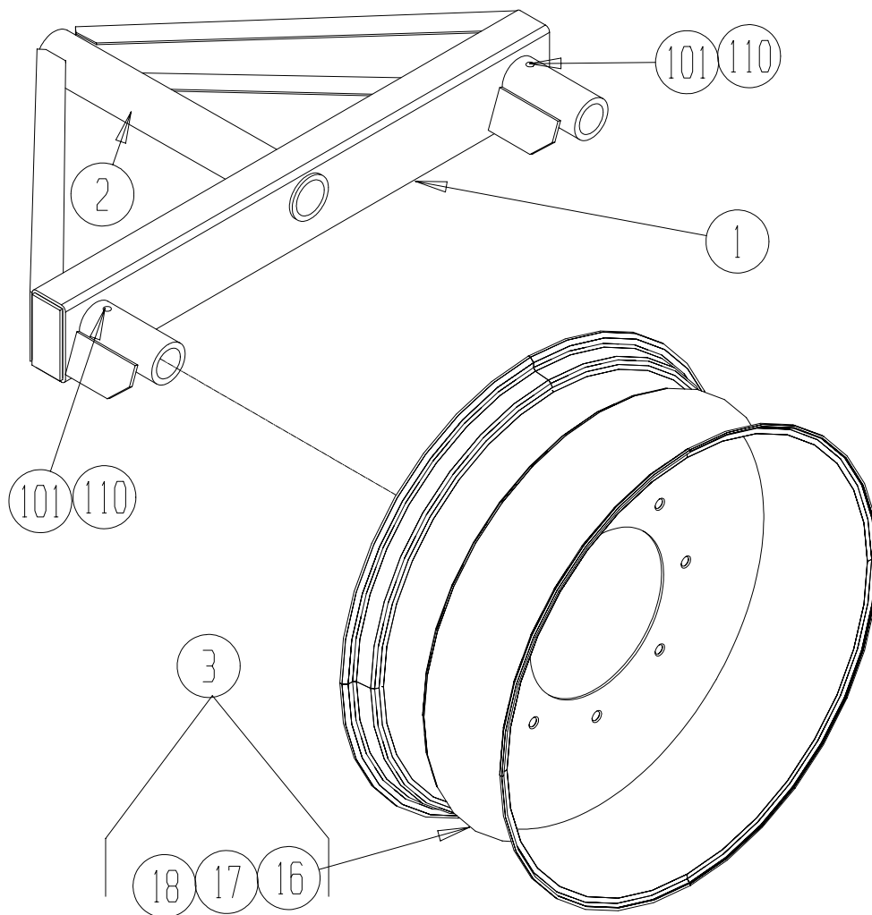
1001-1-9 WHEEL & ROCKER ASSEMBLY
