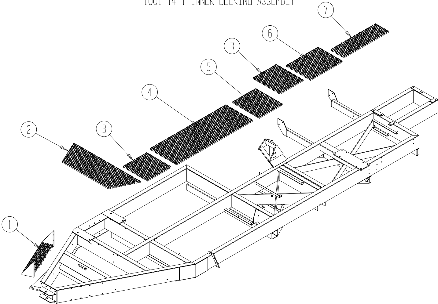
1001-14-1 INNER DECKING ASSEMBLY
