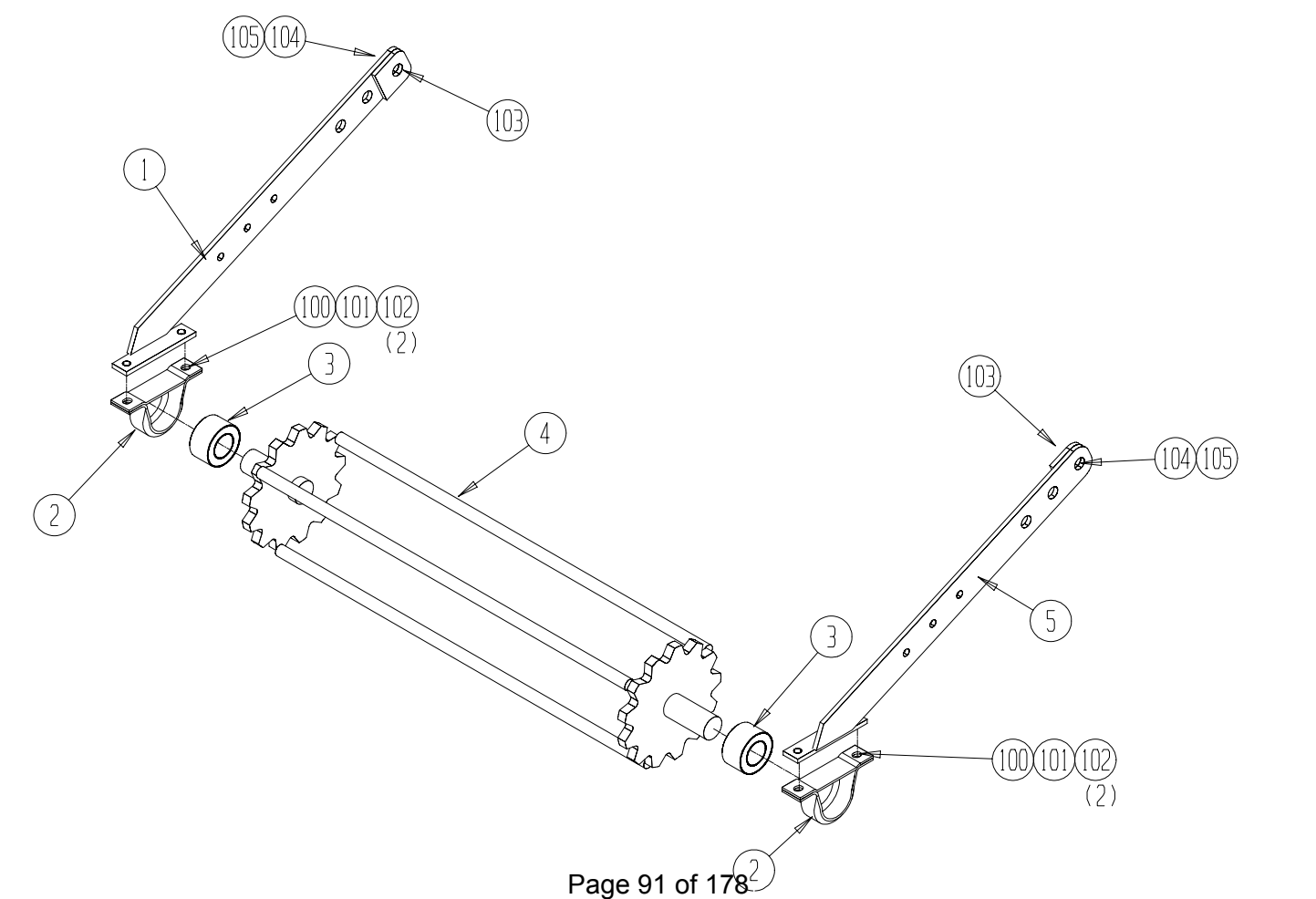
1001-6-4 CROSS CONVEYOR CHAIN CLEANER ASSEMBLY
