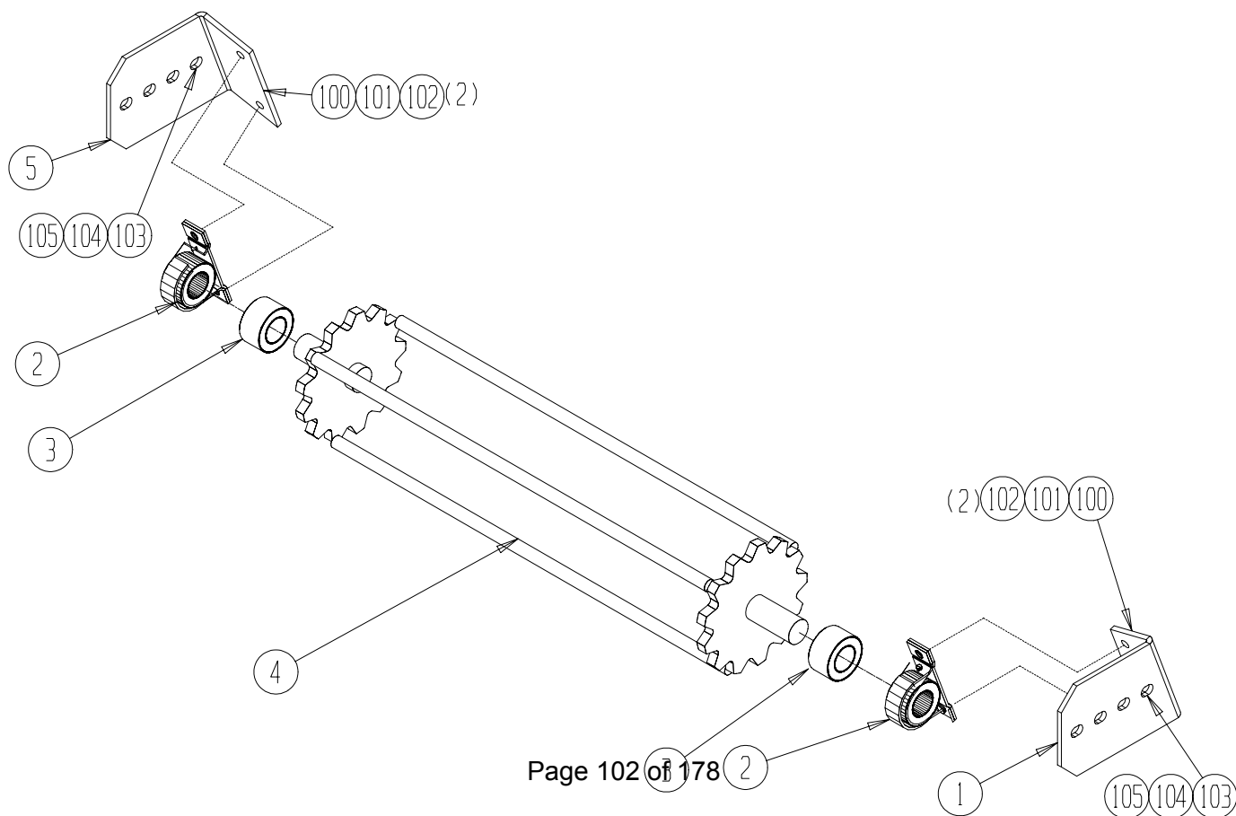
1001-7-4 ELEVATION CONVEYOR BAR CLEANER ASSEMBLY ( KIT-0127 )
