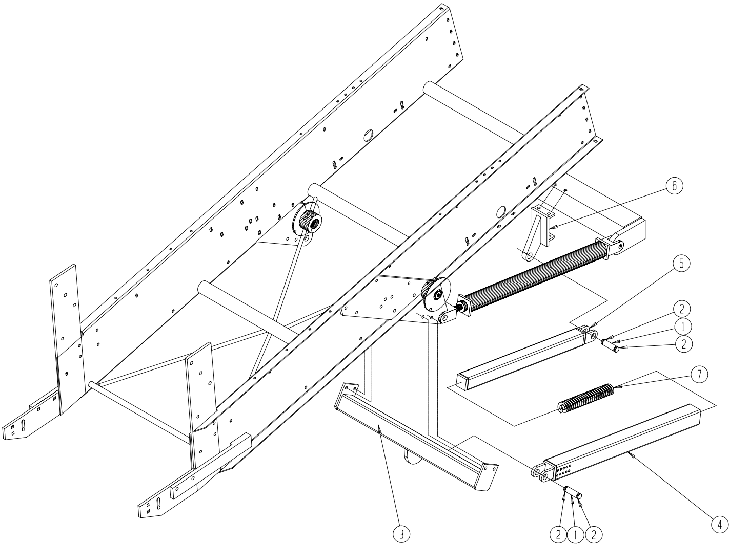
HEADER, SPRING ASSISTED LIFT ASSEMBLY / KIT-0077
