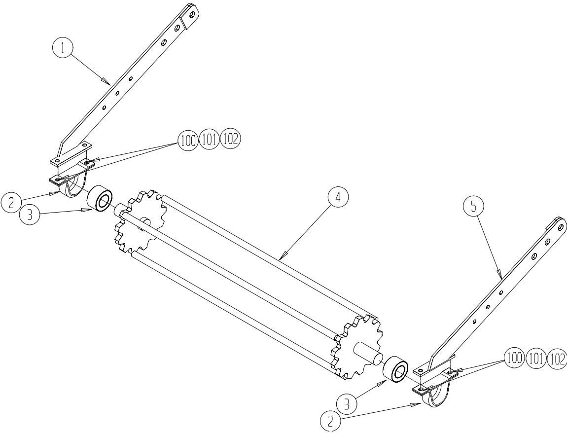
1001-4-4 TRANSFER CHAIN CLEANER ASSEMBLY
