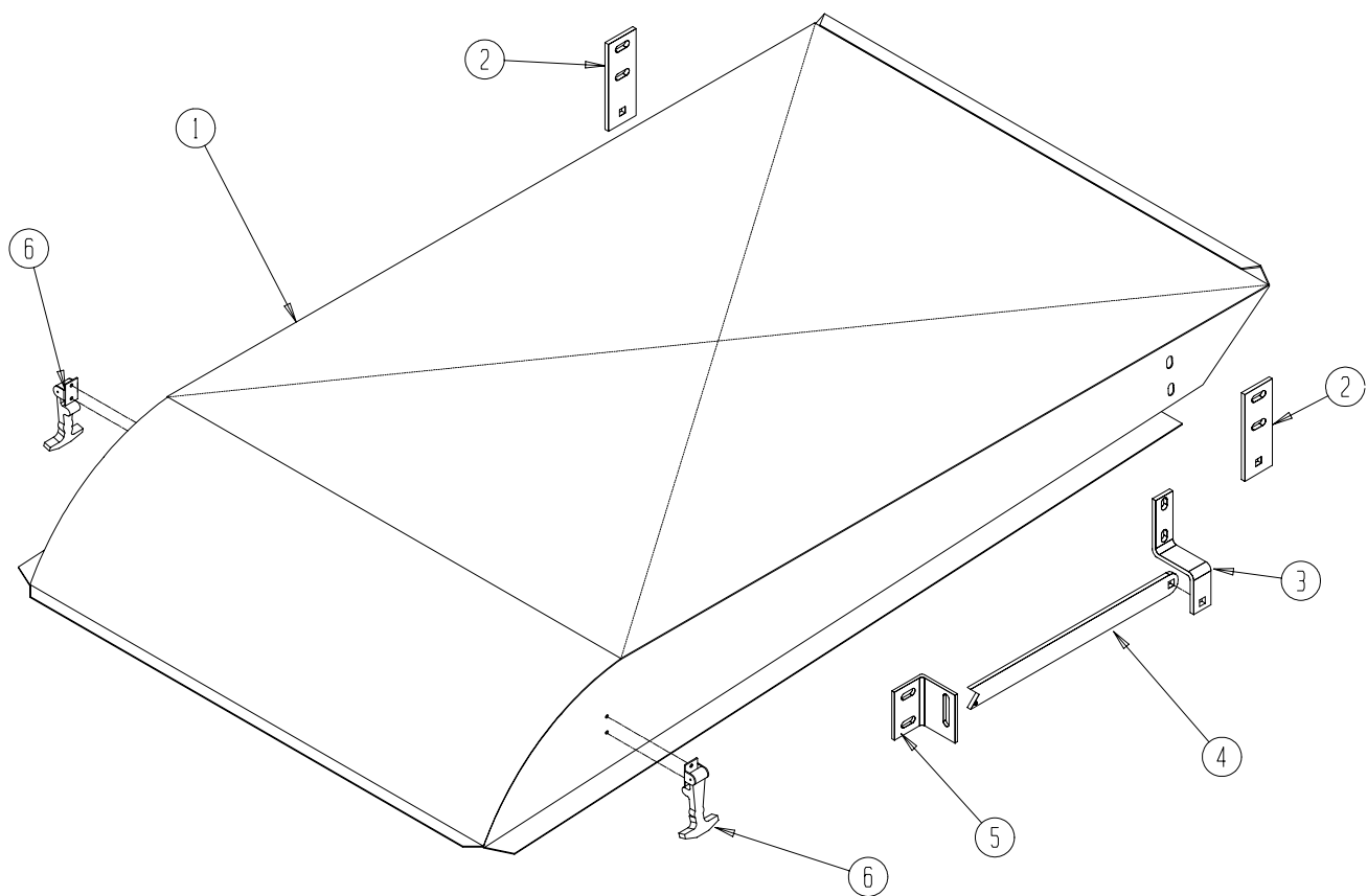
1001-6-6 CROSS CONVEYOR COVER ASSEMBLY
