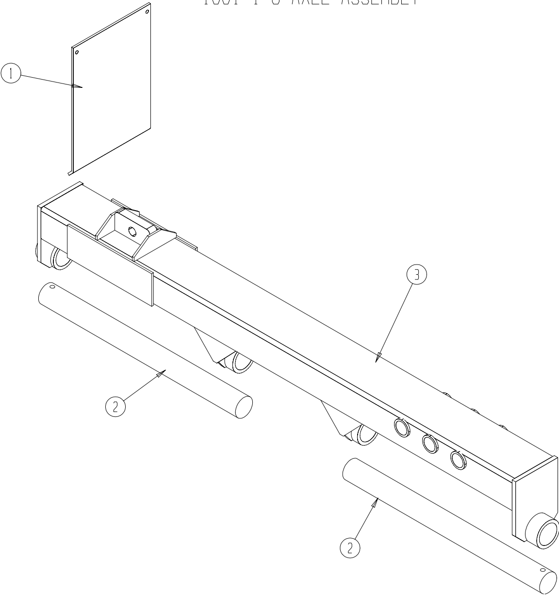
1001-1-8 AXLE ASSEMBLY
